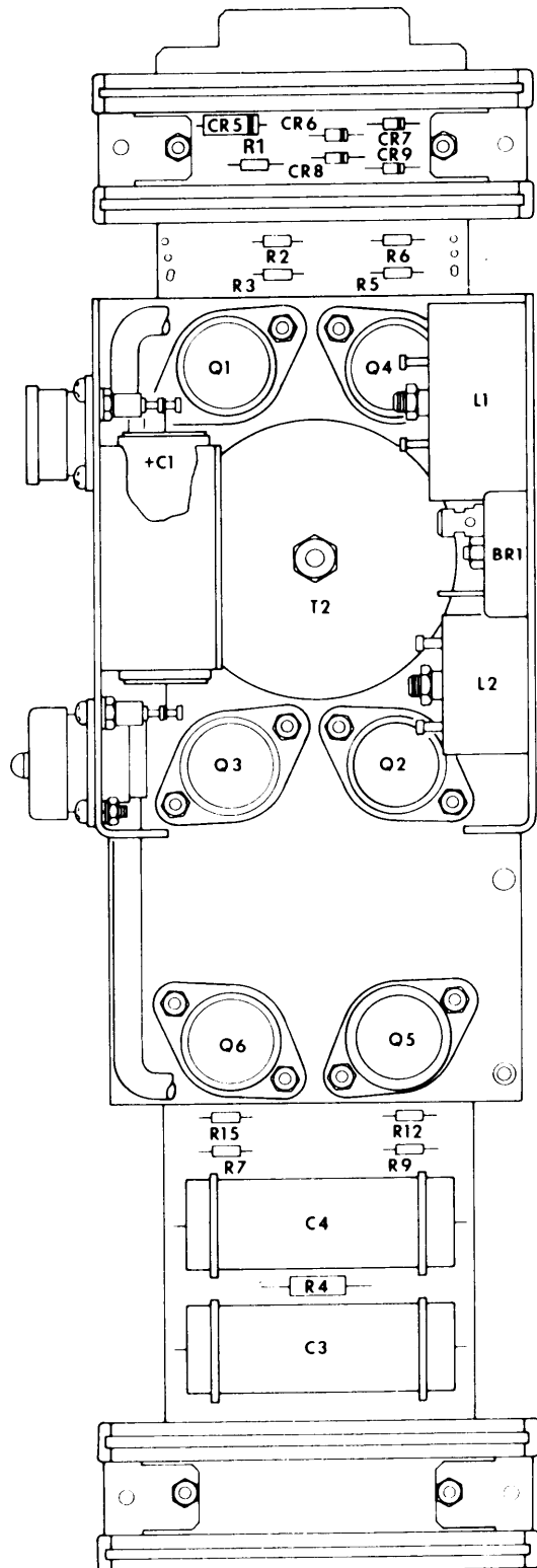
Figure 2-8 Battery Charger/Regulator (1A1A1) -schematic and parts placement. (sheet 2 of 2)
