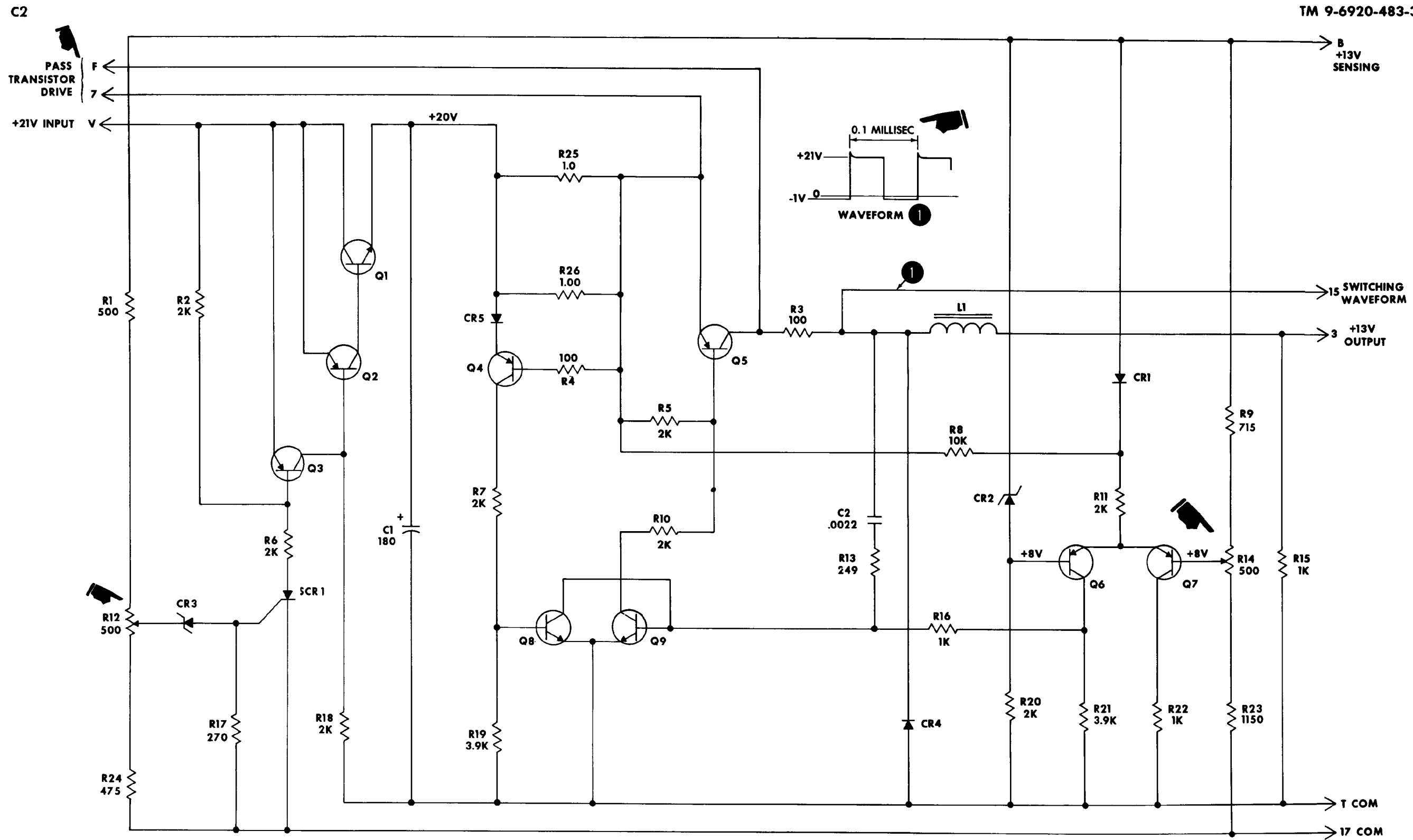
Figure 2-11. Circuit card assembly 1A1A1A4, +13 volt Power Supply -schematic and parts placement. (sheet 1 of 2)
