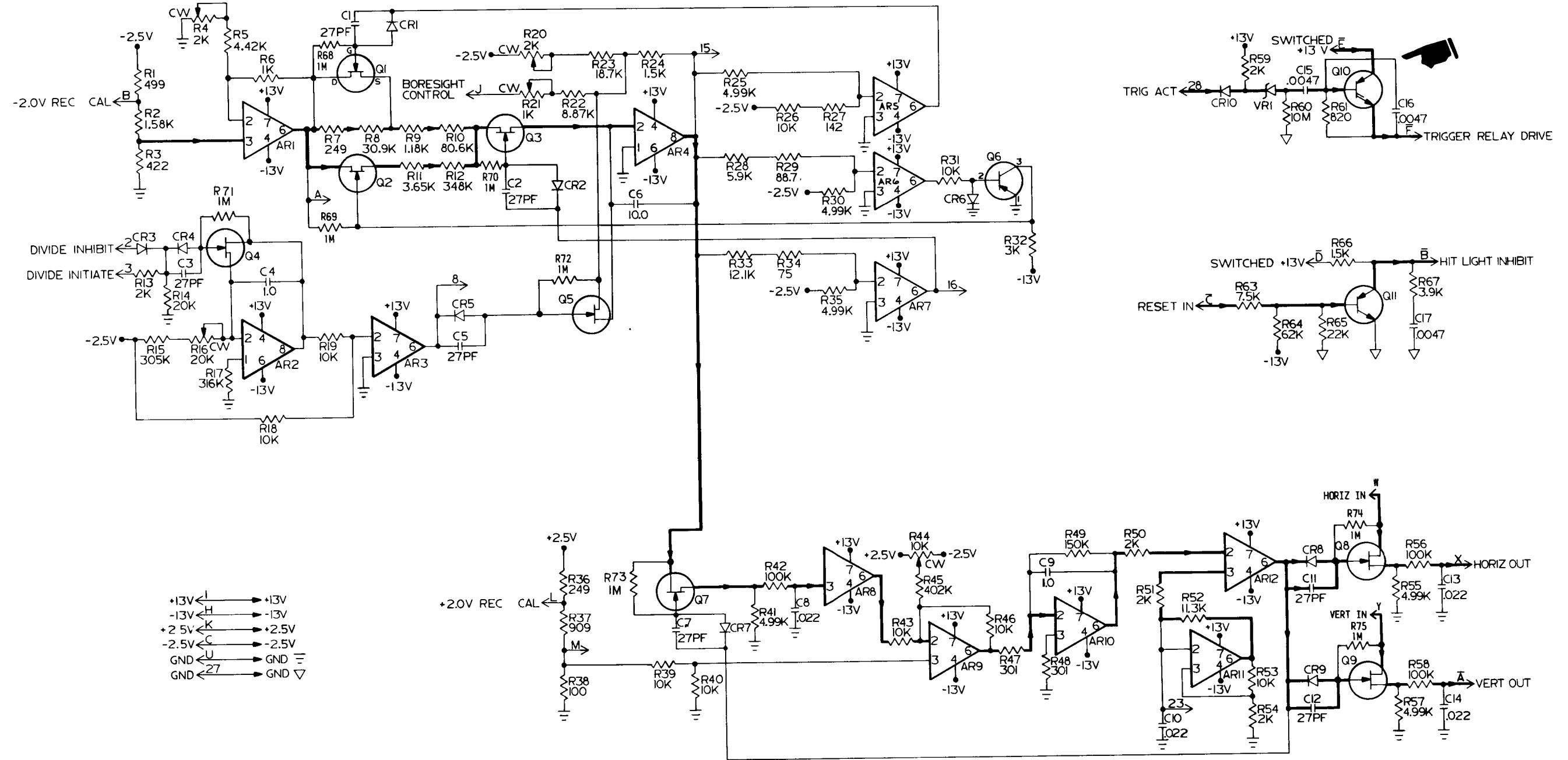
Figure 3-7. 1A1A2A7 printed circuit card-schematic and parts placement. (sheet 1 of 2)
