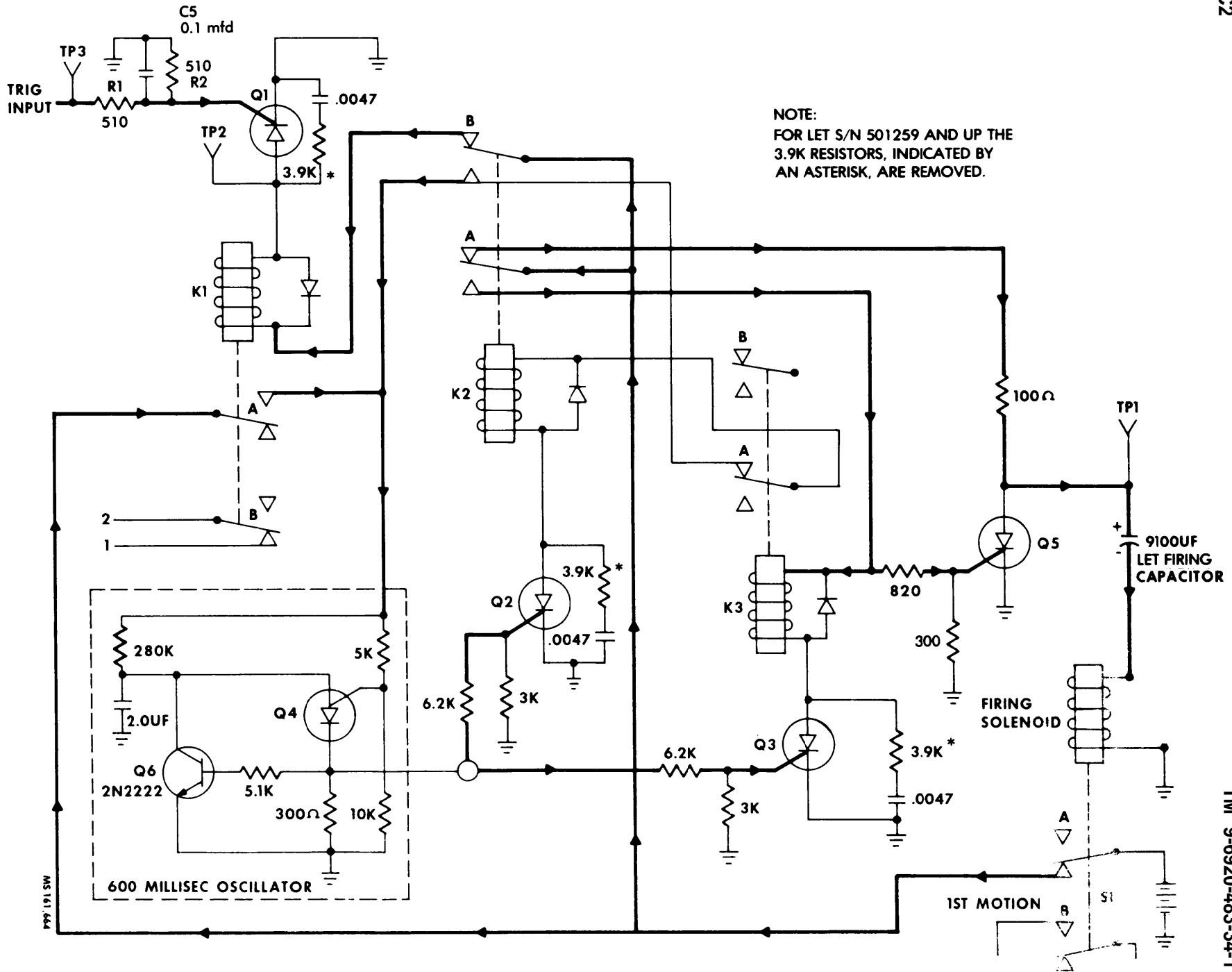
Figure 2-20. Electronic functions of the Trainer
