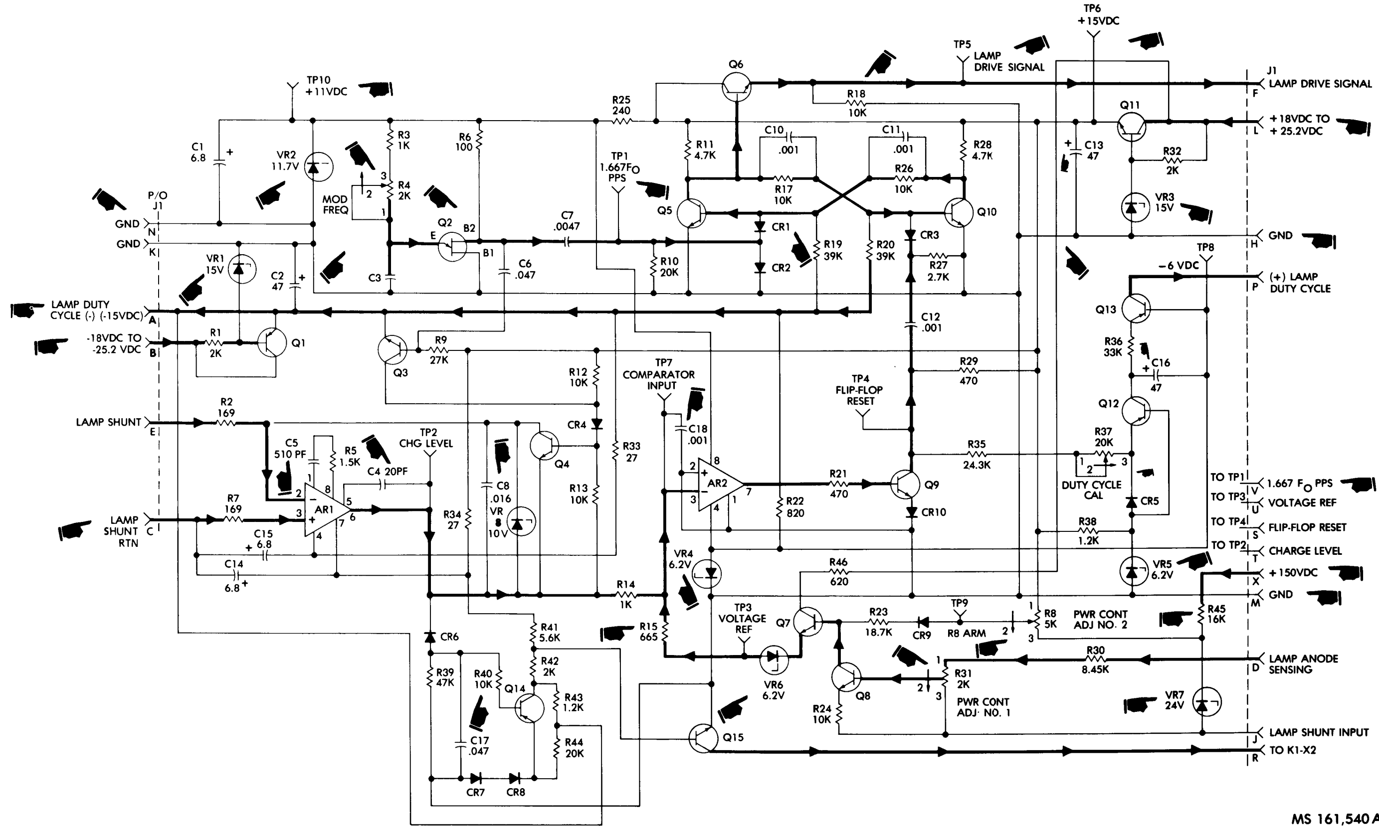
MS 161,540 A Figure 2-18. IR Transmitter Power Control card-11500196
