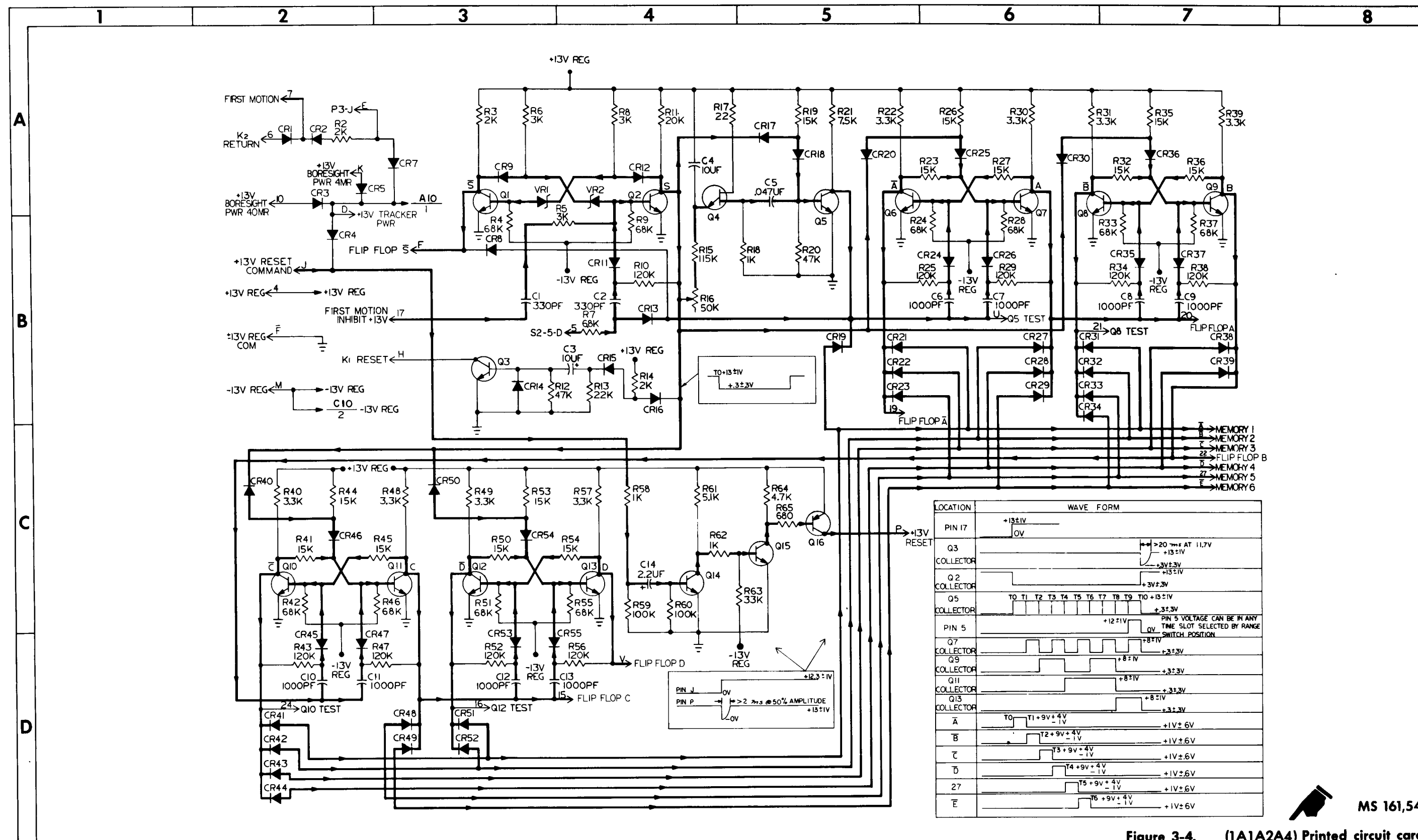
Figure 3-4. (1A1A2A4) Printed circuit card-schematic and parts placement (sheet 1 of 3)
